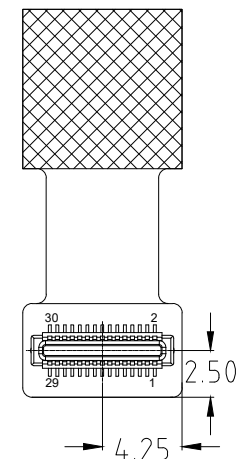
BOTTOM VIEW
